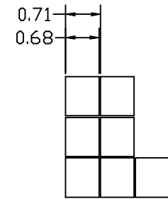
DOT DETAIL
